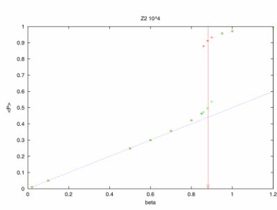
Z2 Gauged Spin Model average plaquette
