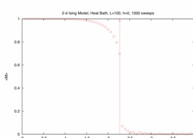
Magnetisation in the Ising Model
