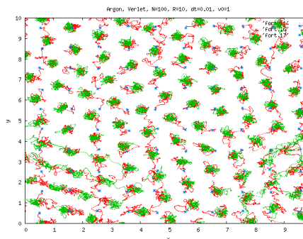
Argon gas Molecular Dynamics, low temp
