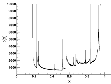
Logistic Map Invariant Density ( \mu=3.8 )
