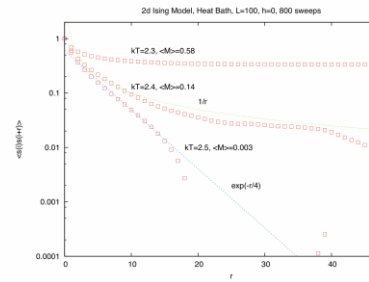
\langle s_i s_{i+r} \rangle Spin-Spin Correlation Function in the Ising Model
