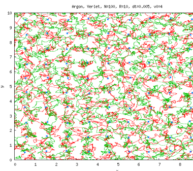
Argon gas Molecular Dynamics, high temp
