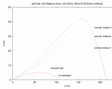
Magnus Force and Golf Balls
