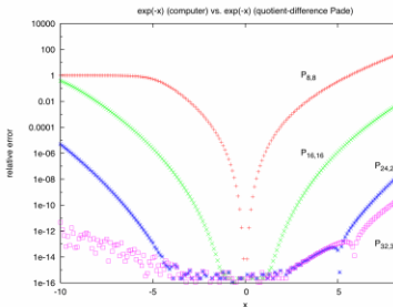
Exponential Function with the Quotient-Difference Algorithm and Pade Approximants
