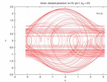
Damped, Driven Oscillator Phase Map
