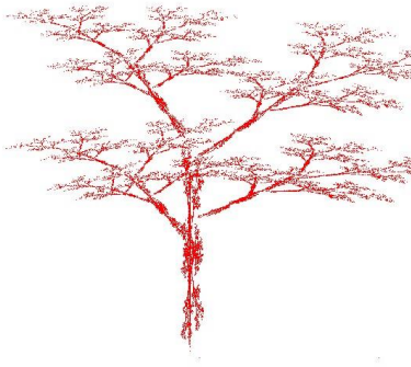
Affine Map
