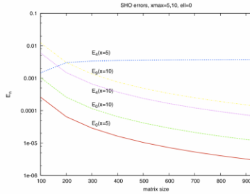
Accuracy in S-wave SHO eigenvalues
