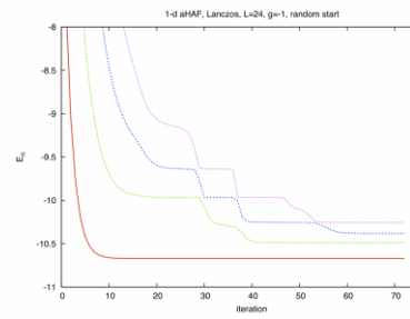
1-d anisotropic Heisenberg Antiferromagnet spin chain, L=24 , g=-1
