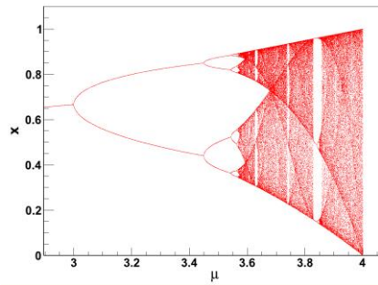
Logistic Map Bifurcation Plot
