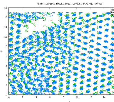
Argon Molecular Dynamics, Emergent Disorder
