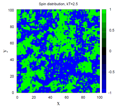
Ising Spins at kT = 2.5
